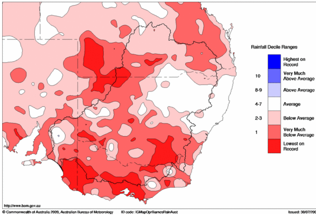
Figure 2. Rainfall deciles for the Murray-Darling Basin, for 8 years from 1 st July 2001 to 30 th June 2009. (source: Bureau of Meteorology)
