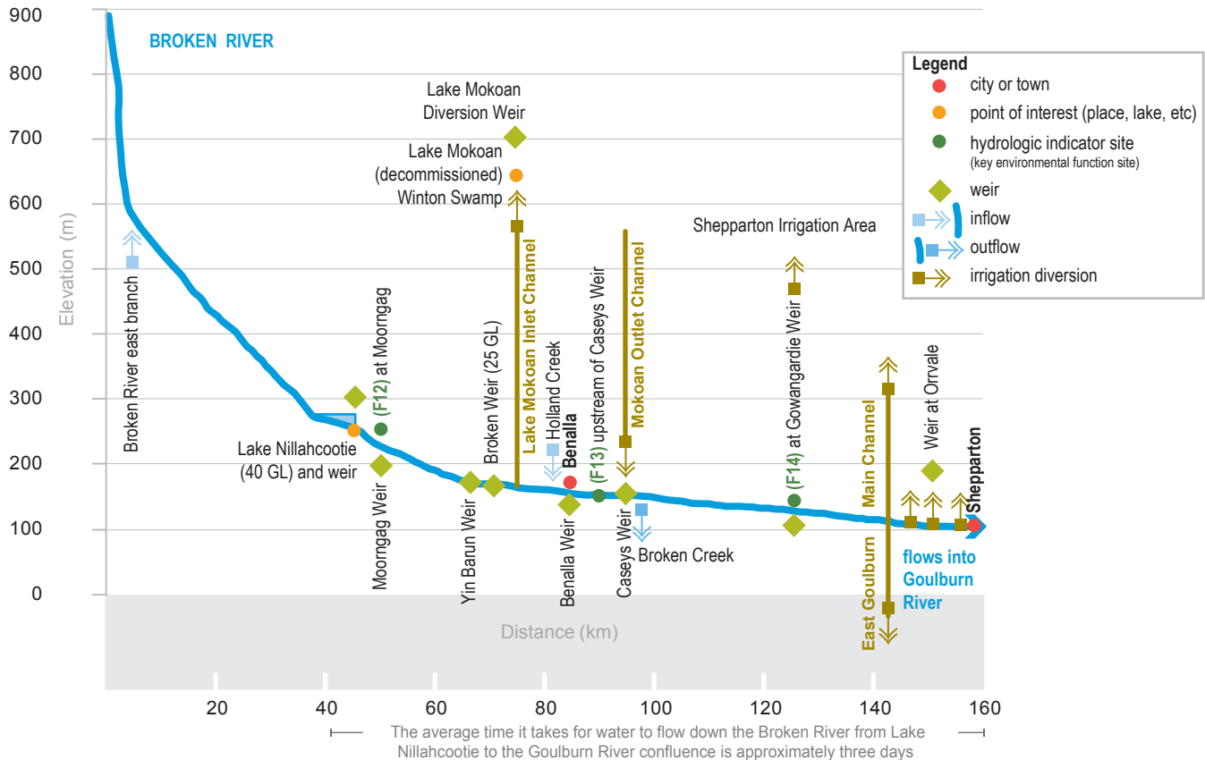
Figure 2 Broken River longitudinal profile
