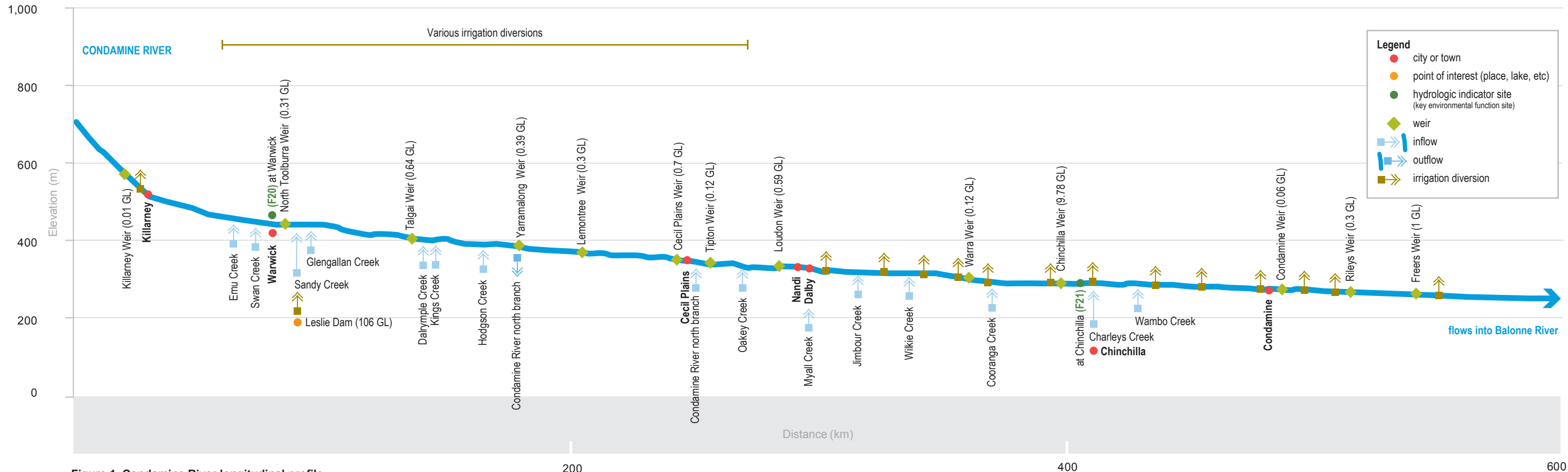
Figure 1 Condamine River longitudinal profile
