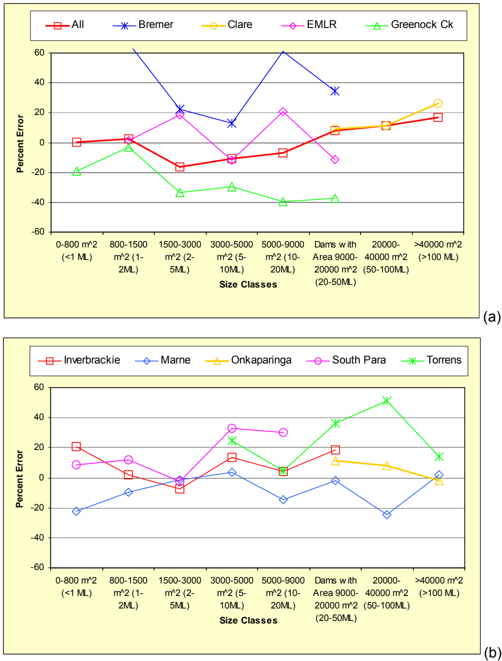
Figure 4.10 Errors in size classes obtained when Relationship 4.1 was applied to data from each catchment individually and to all data combined.
